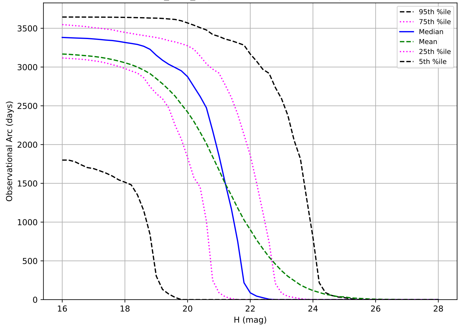
baseline_v3.5_10yrs: Observational Arc Length NEO
