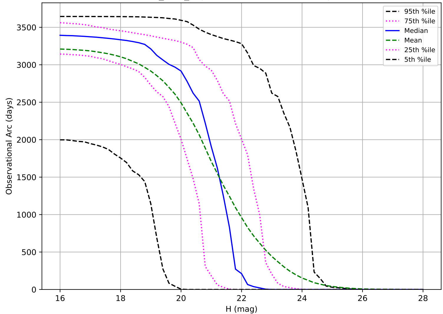
baseline_v3.5_10yrs: Observational Arc Length PHA
