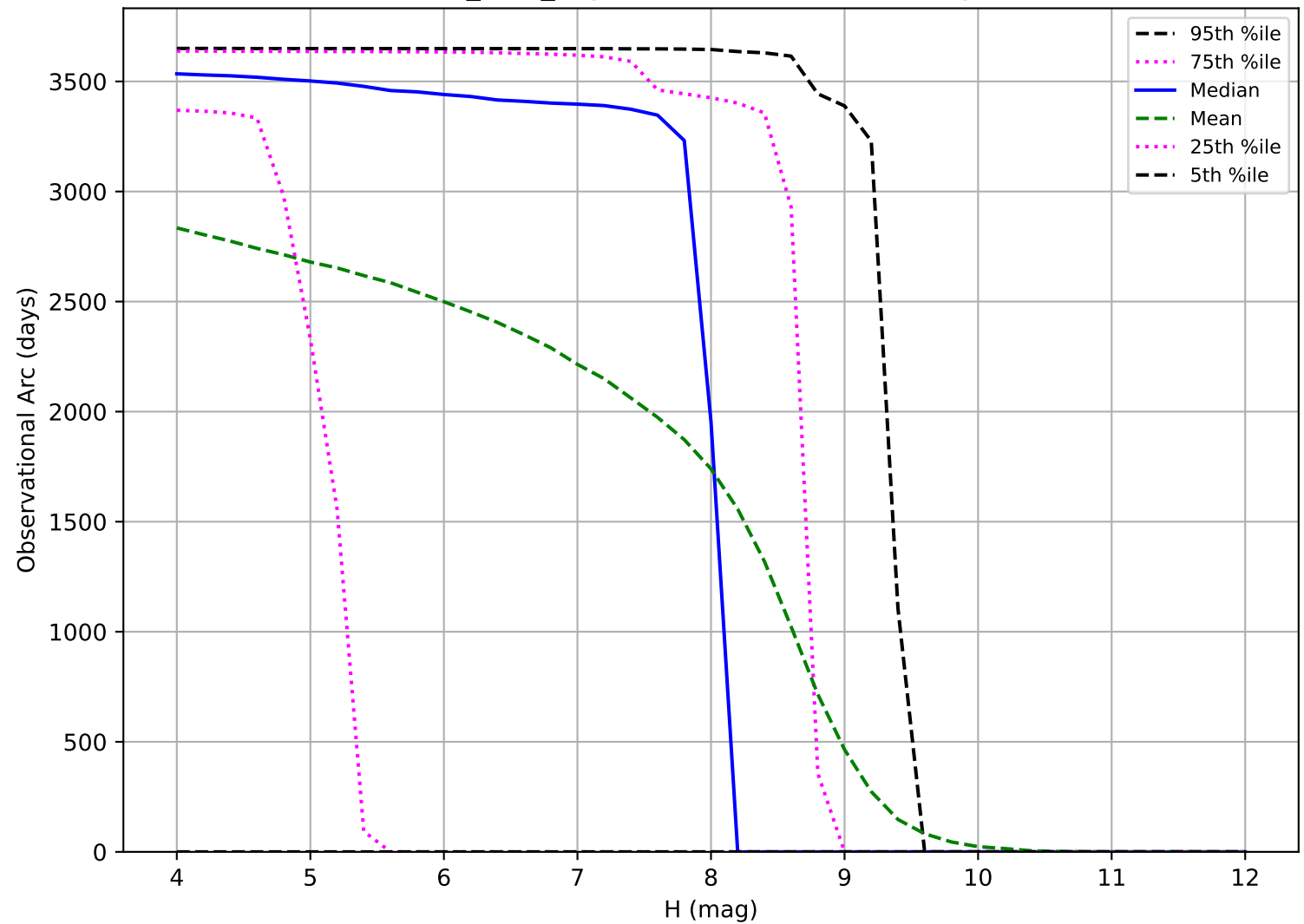
baseline_v3.5_10yrs: Observational Arc Length TNO
