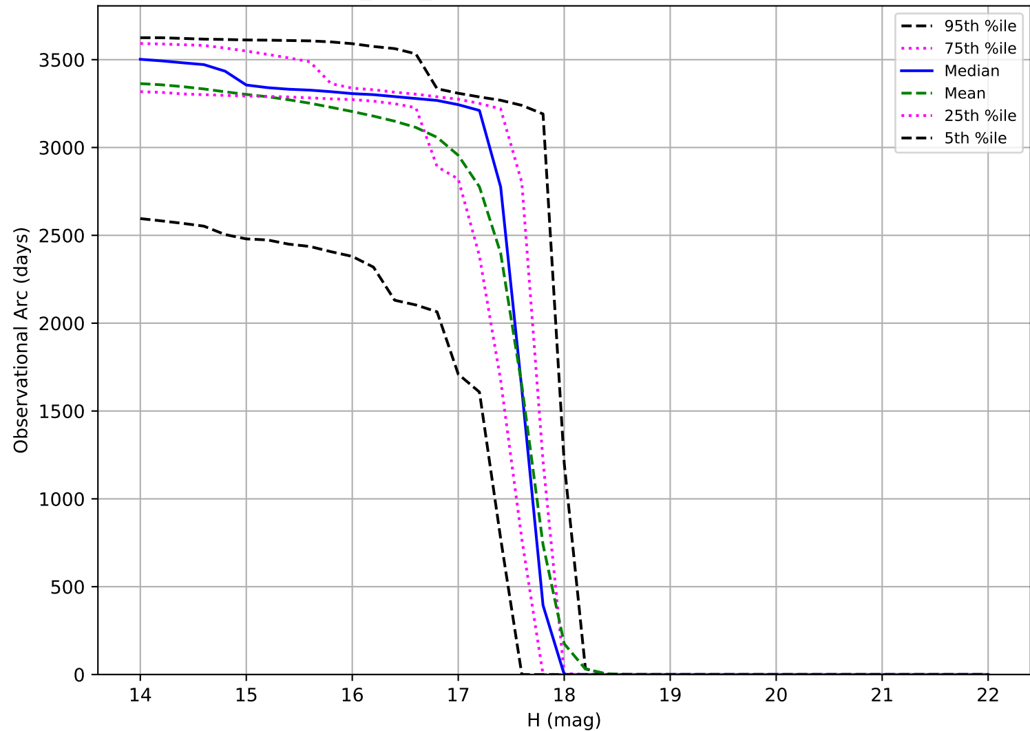
baseline_v3.5_10yrs: Observational Arc Length Trojan
