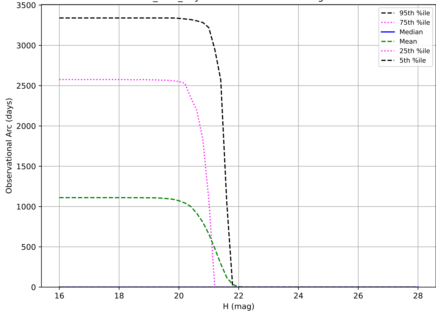
baseline_v3.5_10yrs: Observational Arc Length Vatira
