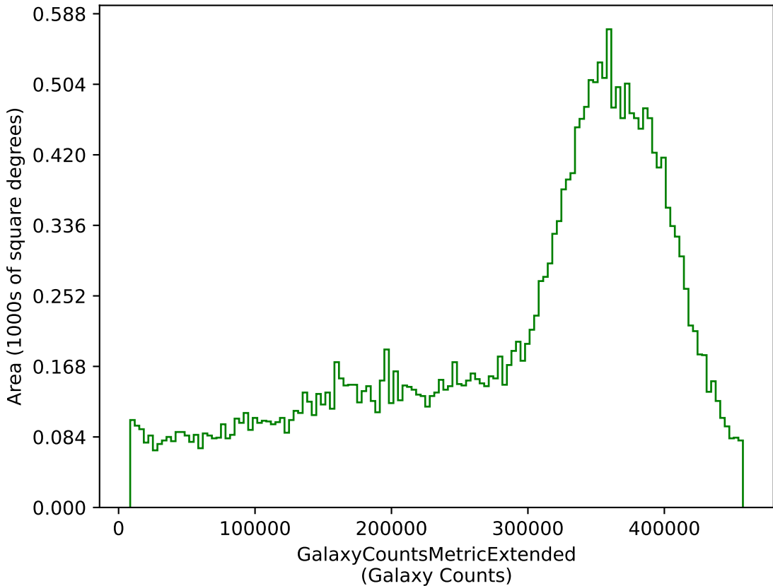
baseline_v3.6_10yrs g: GalaxyCountsMetricExtended
