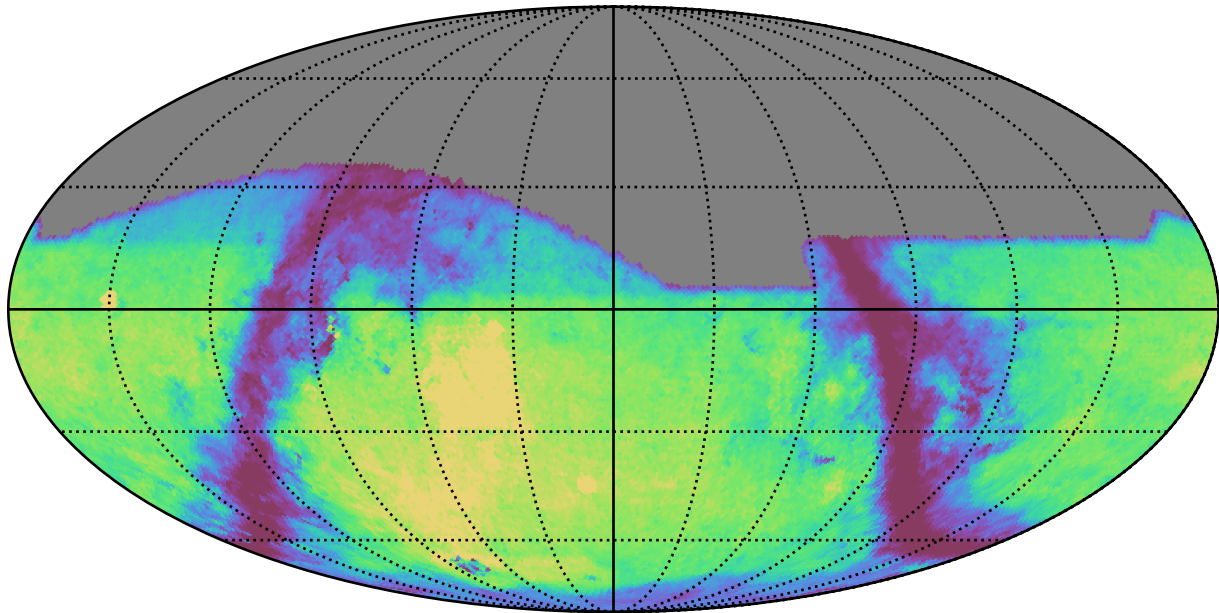
baseline_v3.6_10yrs g: GalaxyCountsMetricExtended
