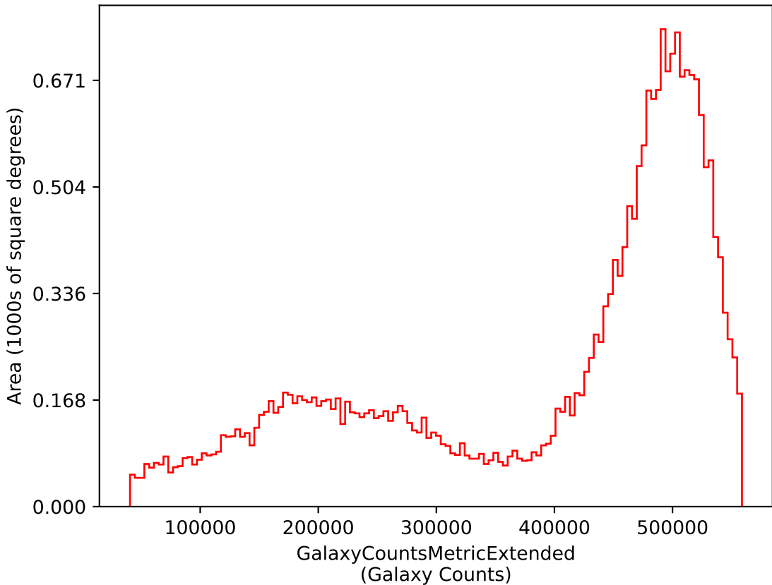
baseline_v3.6_10yrs i: GalaxyCountsMetricExtended
