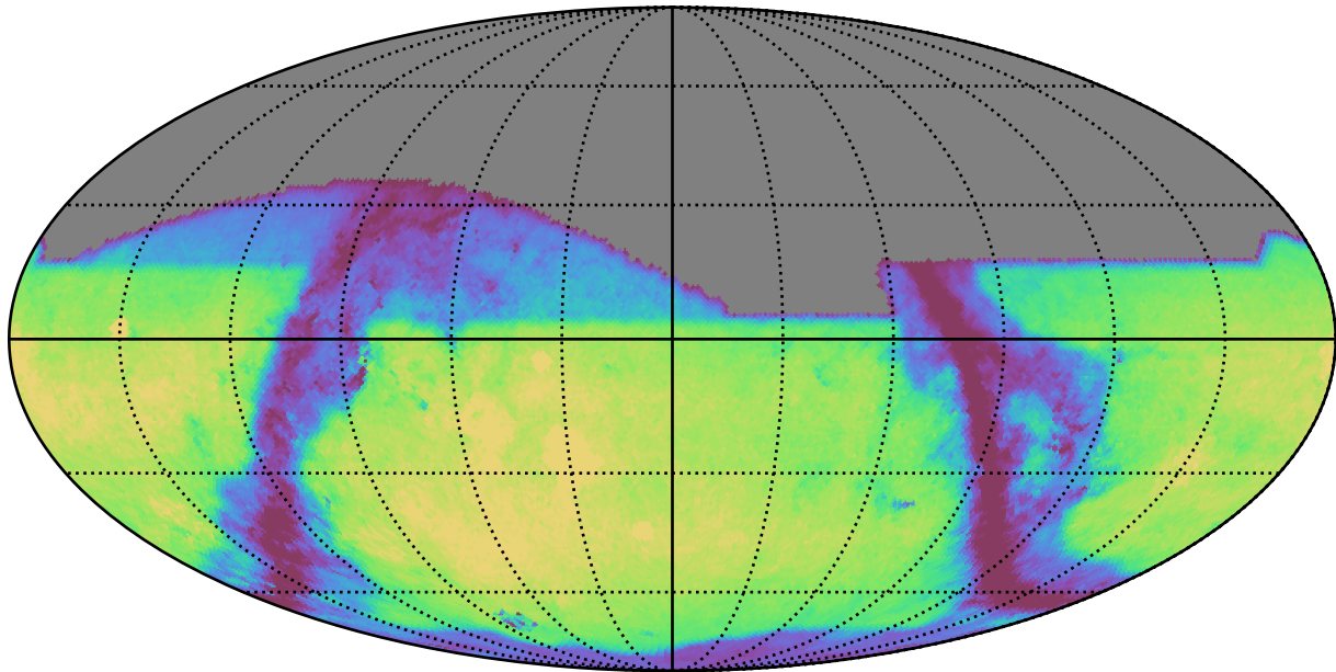
baseline_v3.6_10yrs i: GalaxyCountsMetricExtended
