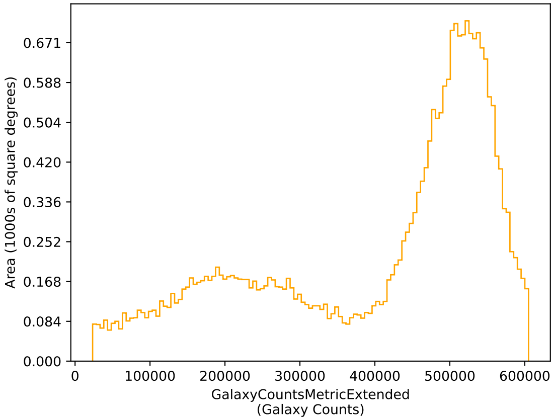
baseline_v3.6_10yrs r: GalaxyCountsMetricExtended
