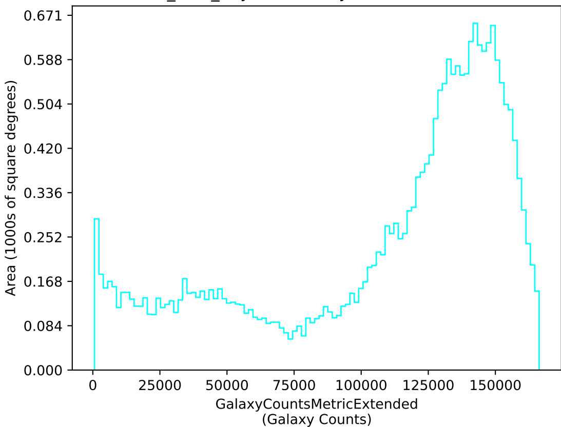
baseline_v3.6_10yrs u: GalaxyCountsMetricExtended
