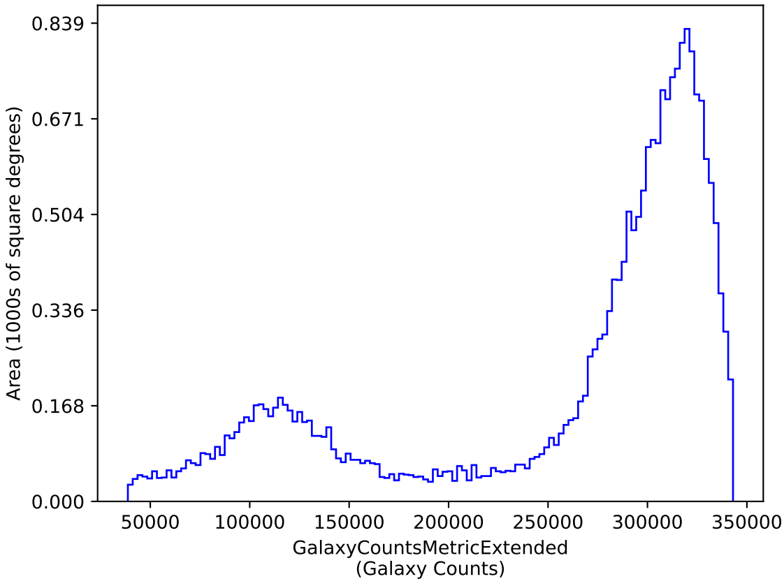
baseline_v3.6_10yrs y: GalaxyCountsMetricExtended
