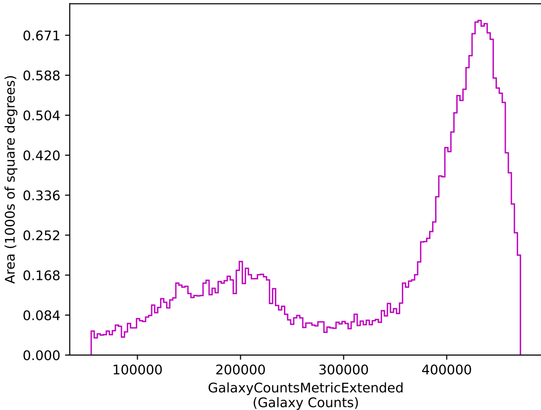
baseline_v3.6_10yrs z: GalaxyCountsMetricExtended
