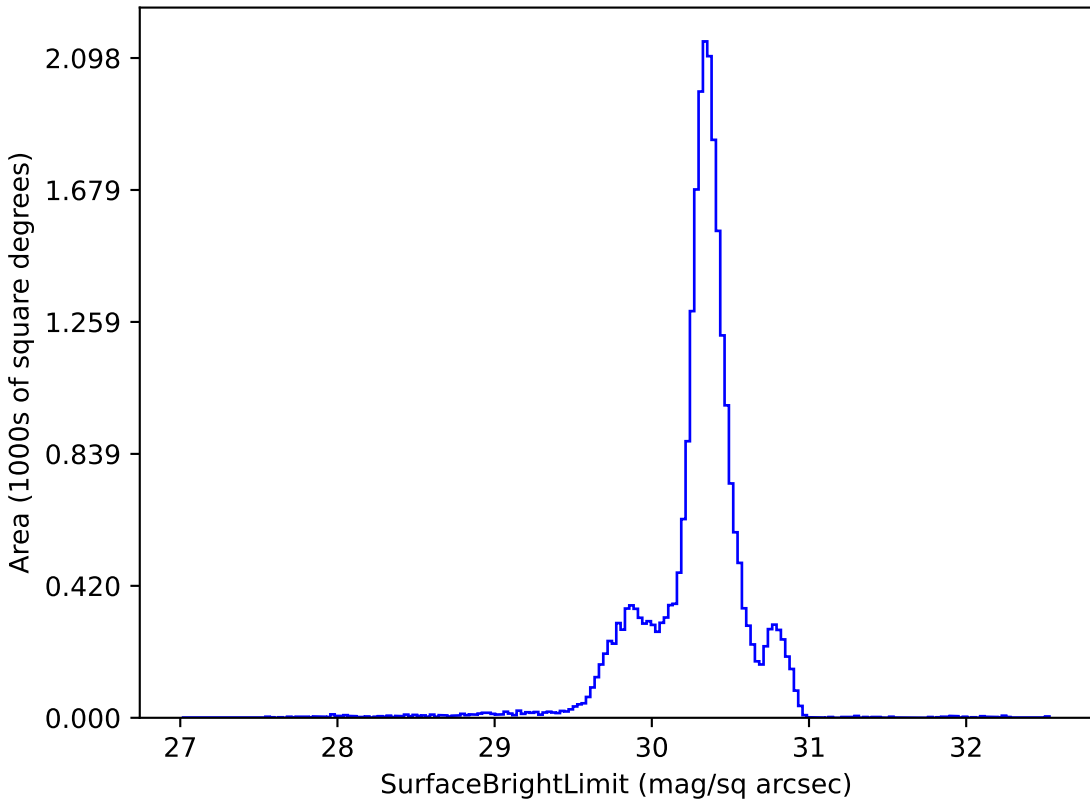
baseline_v3.6_10yrs g: SurfaceBrightLimit
