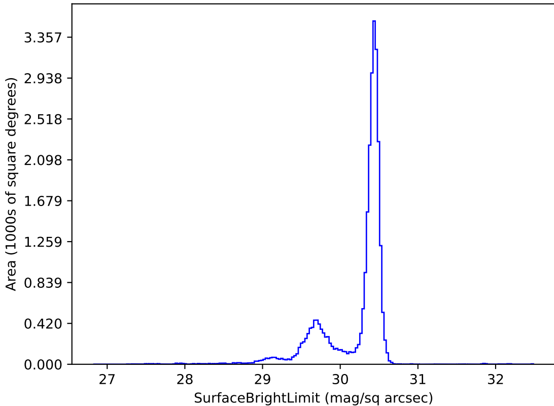
baseline_v3.6_10yrs r: SurfaceBrightLimit
