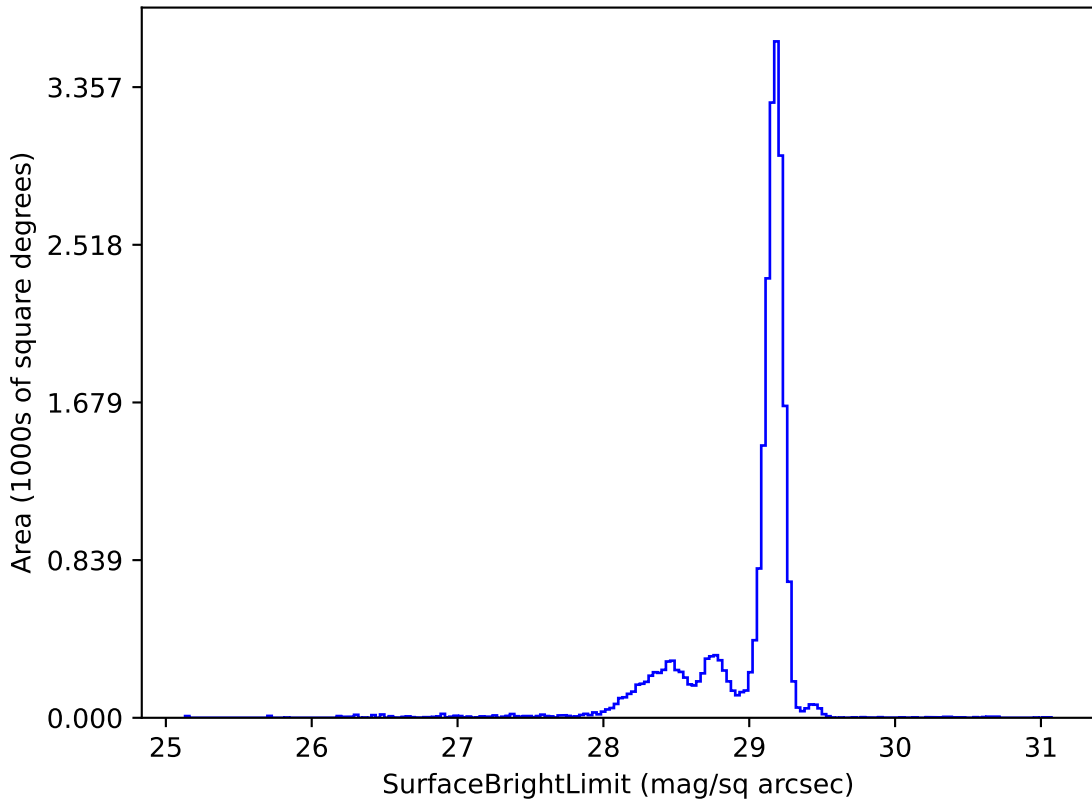
baseline_v3.6_10yrs u: SurfaceBrightLimit
