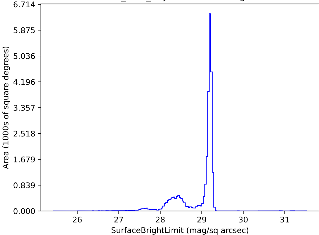
baseline_v3.6_10yrs z: SurfaceBrightLimit
