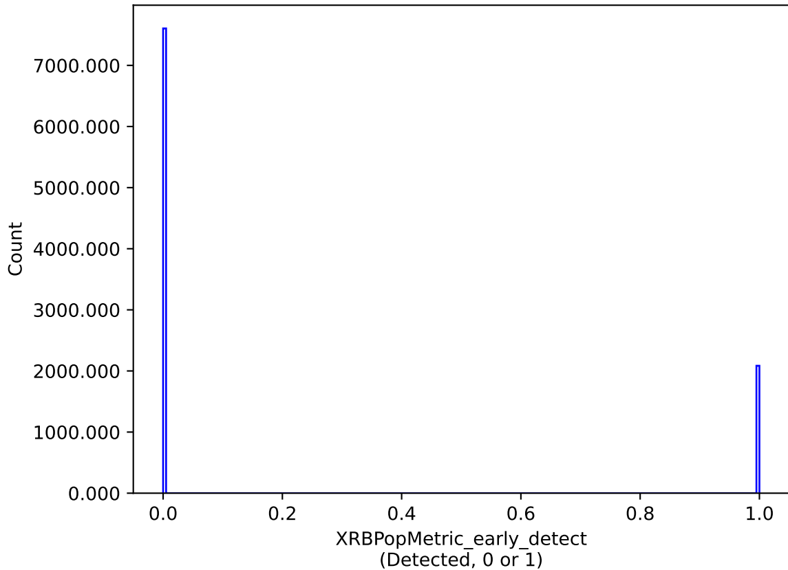
baseline_v3.6_10yrs : XRBPopMetric_early_detect
