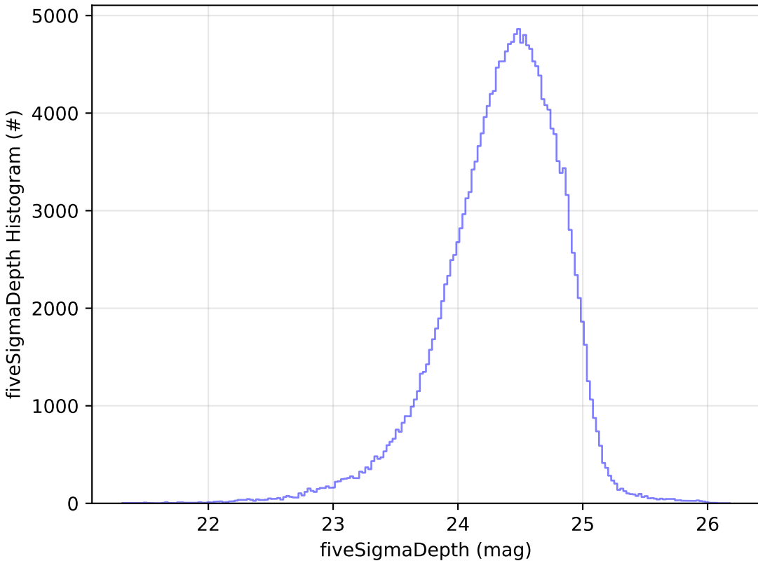
baseline_v3.6_10yrs g: fiveSigmaDepth Histogram
