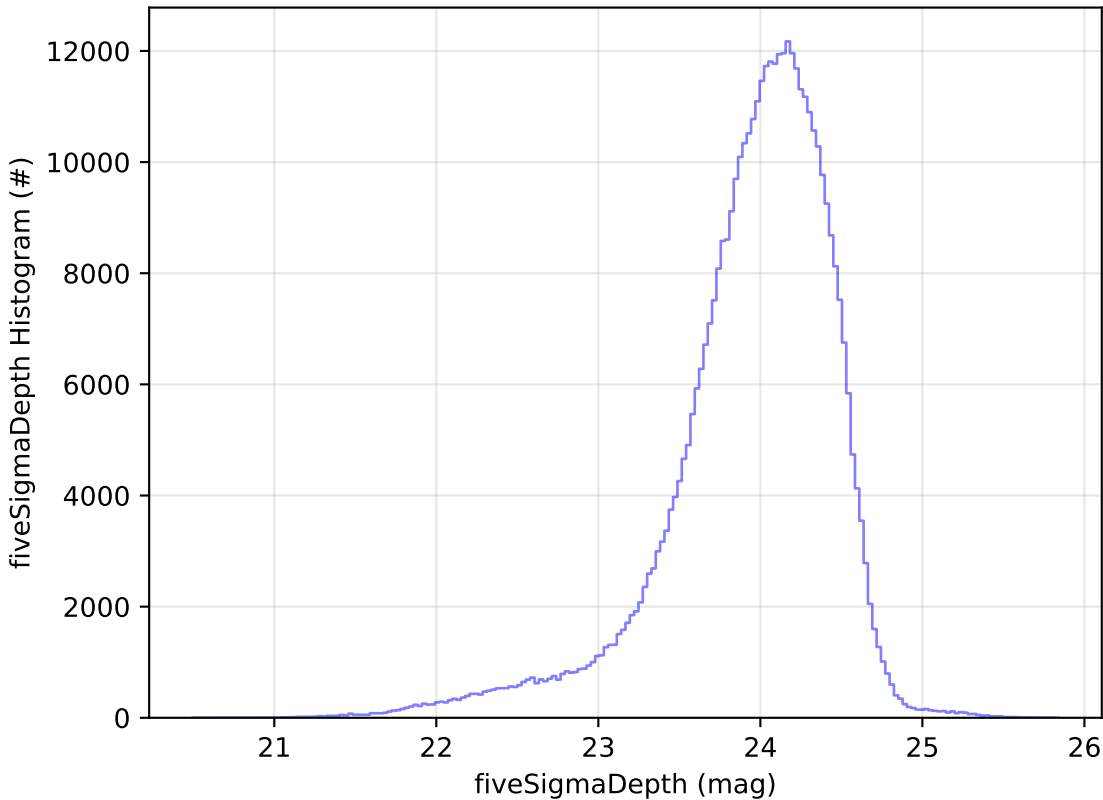
baseline_v3.6_10yrs r: fiveSigmaDepth Histogram
