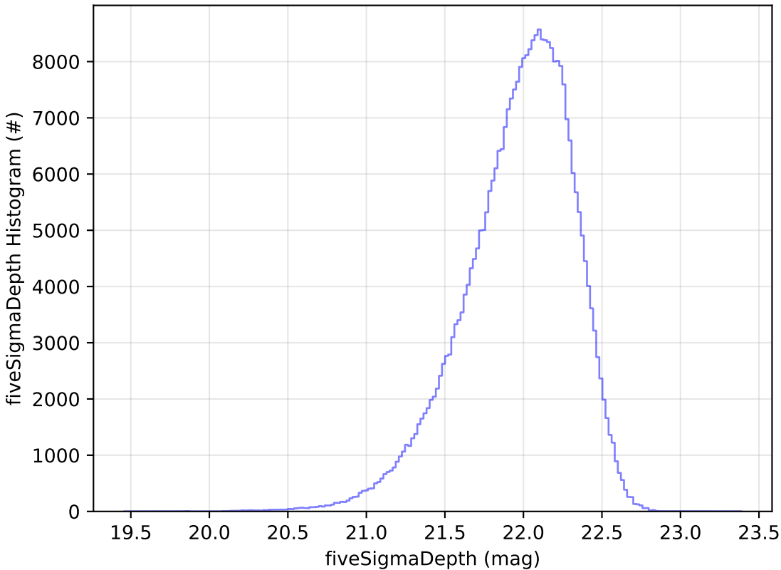
baseline_v3.6_10yrs y: fiveSigmaDepth Histogram
