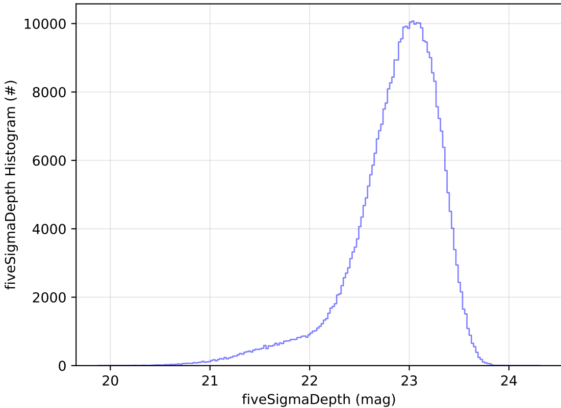
baseline_v3.6_10yrs z: fiveSigmaDepth Histogram
