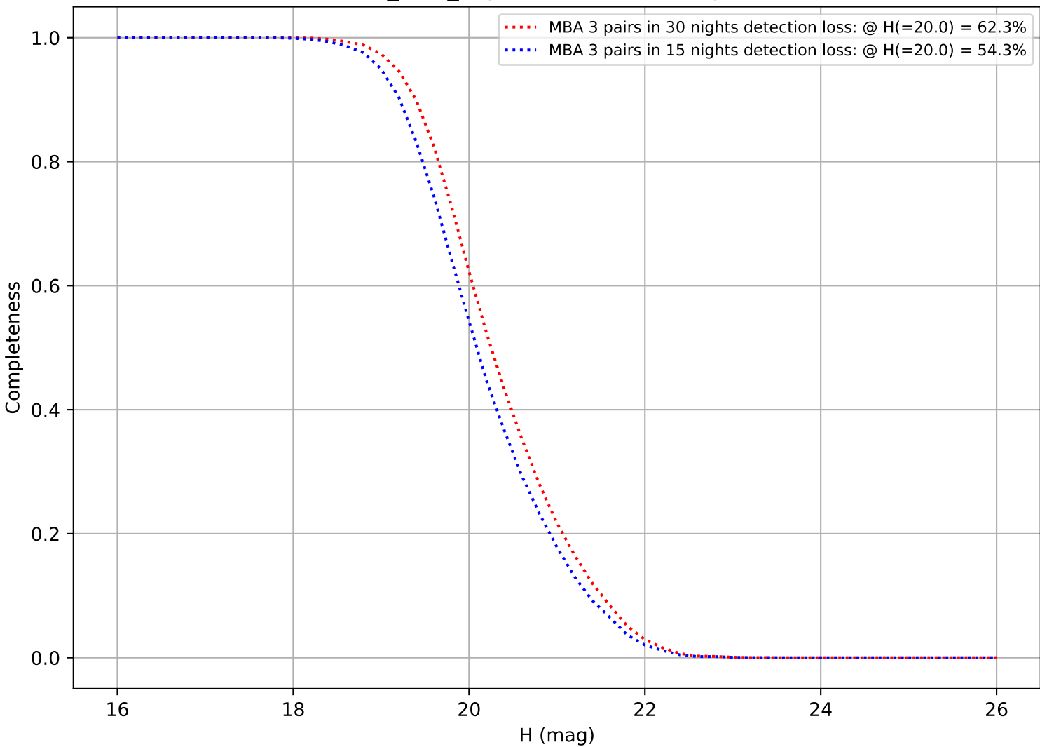
baseline_v3.6_10yrs: DifferentialCompleteness
