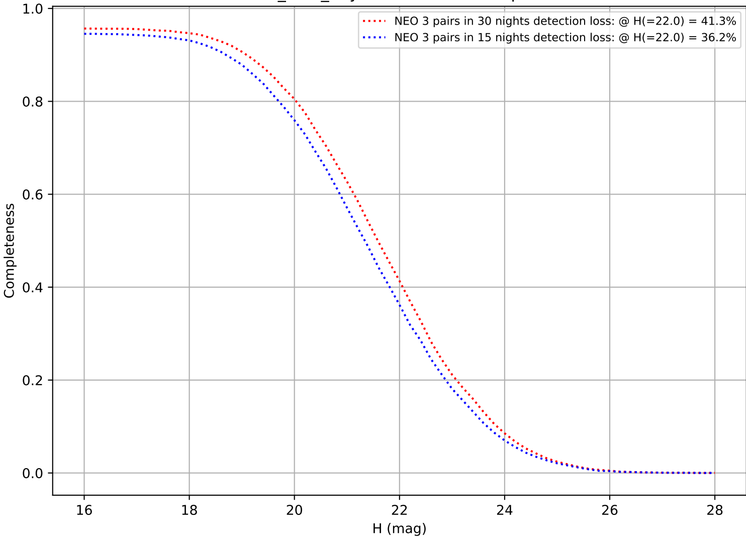
baseline_v3.6_10yrs: DifferentialCompleteness
