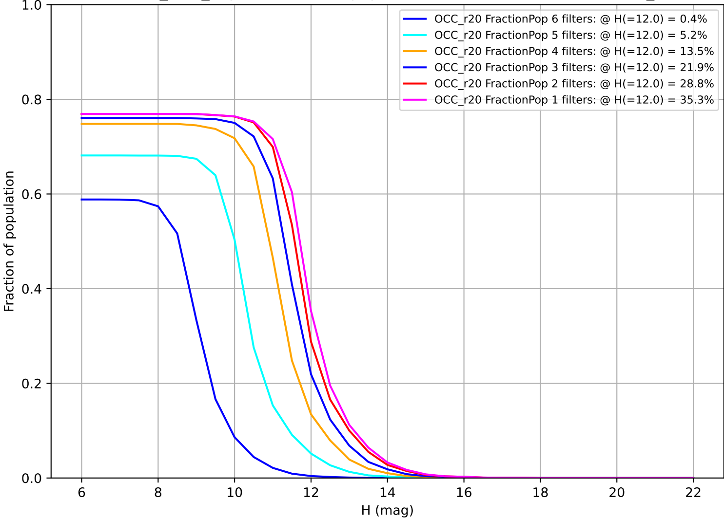
baseline_v3.6_10yrs: Fraction of population with colors in X filters OCC_r20
