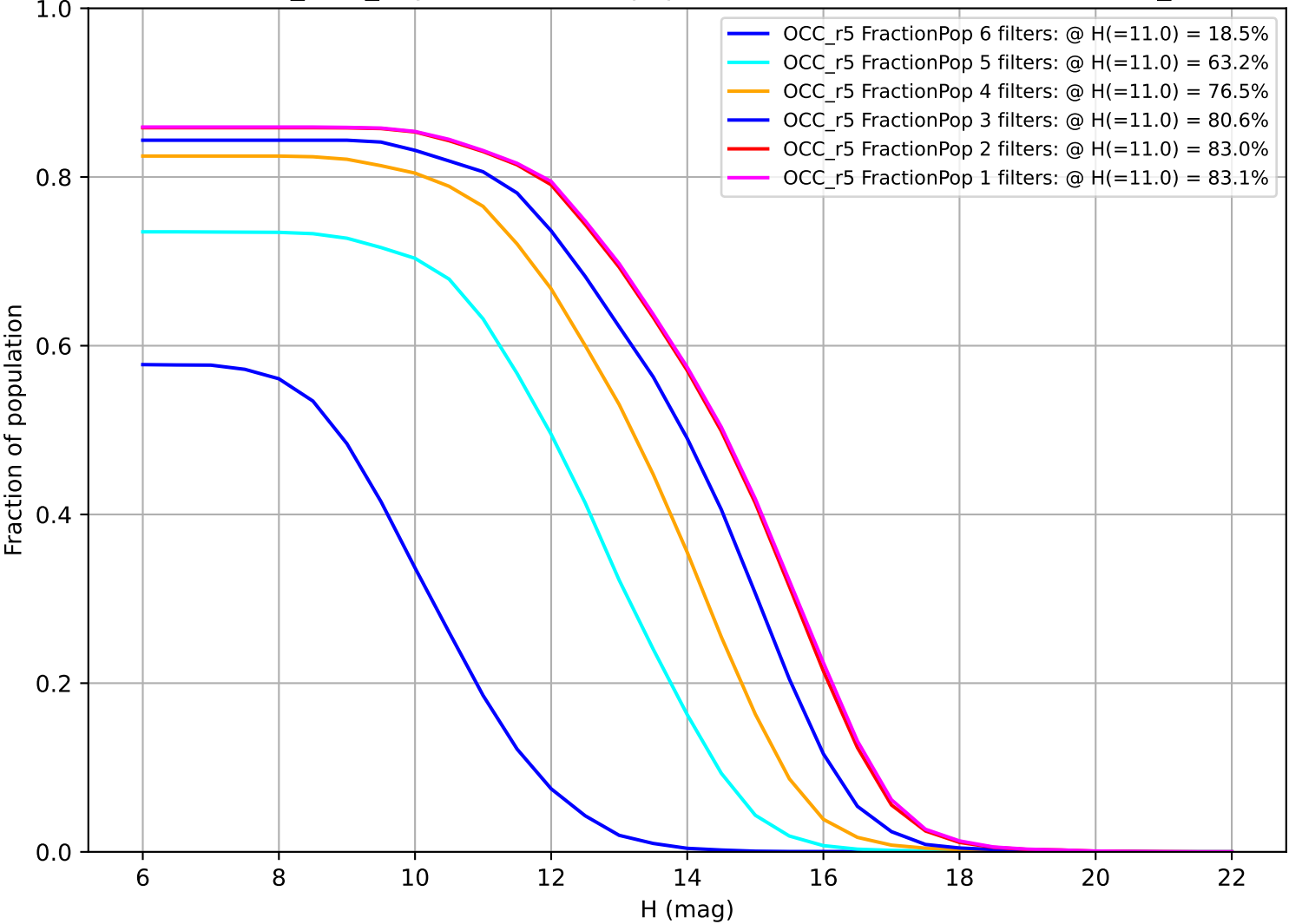
baseline_v3.6_10yrs: Fraction of population with colors in X filters OCC_r5
