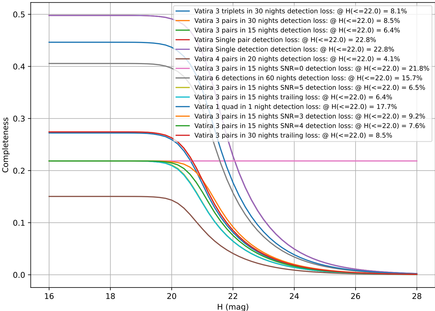
baseline_v3.6_10yrs: CumulativeCompleteness
