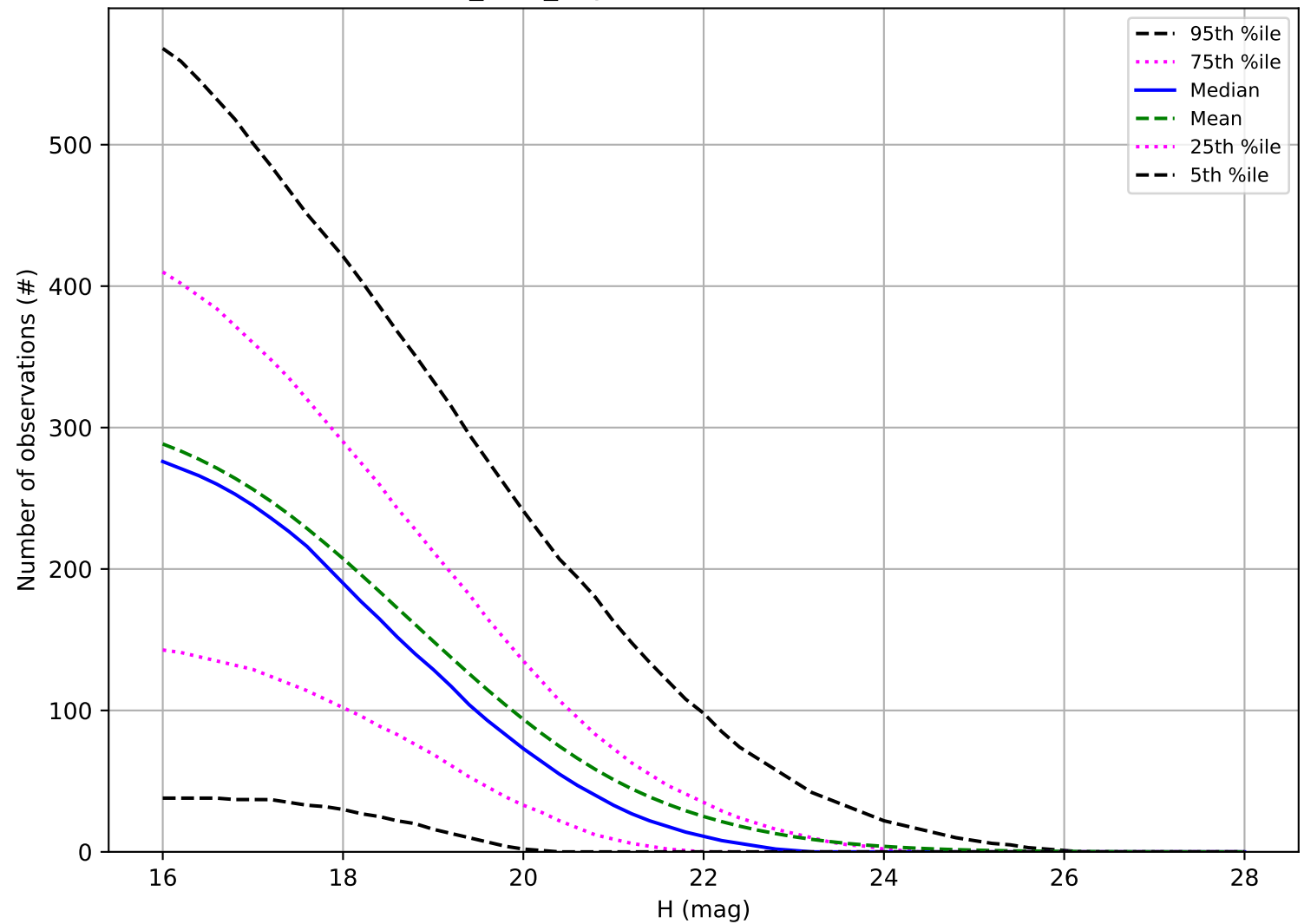
baseline_v3.6_10yrs: Number of observations PHA
