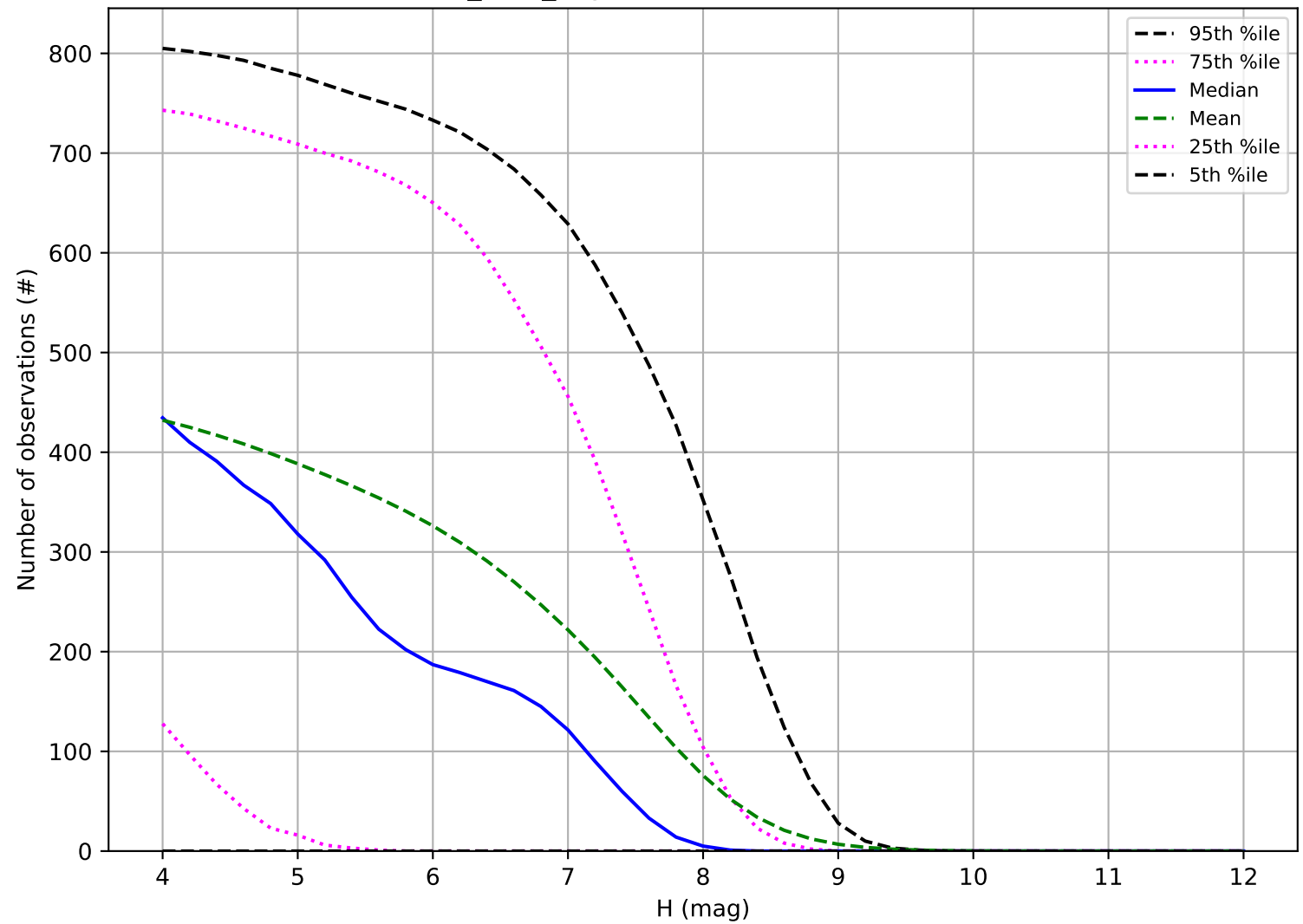
baseline_v3.6_10yrs: Number of observations TNO
