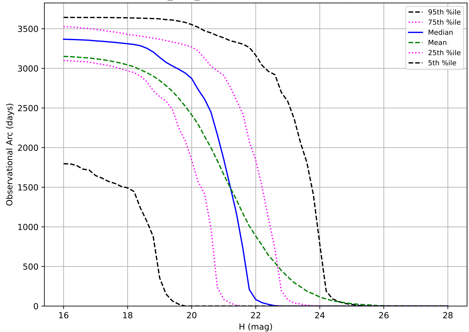
baseline_v3.6_10yrs: Observational Arc Length NEO
