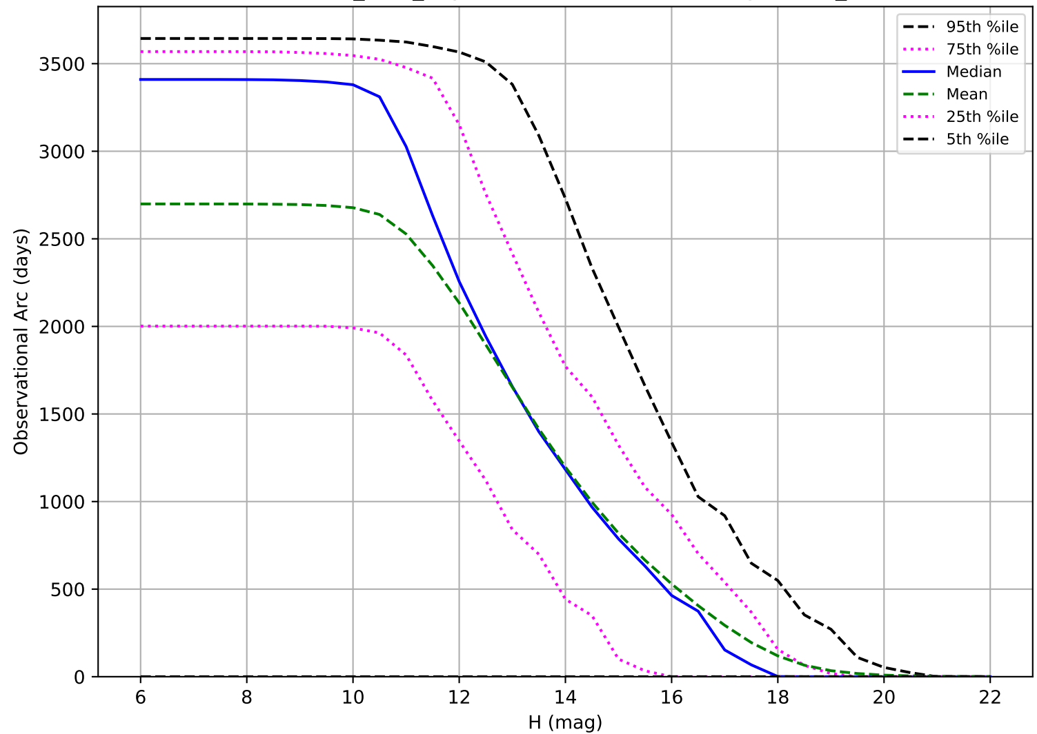
baseline_v3.6_10yrs: Observational Arc Length OCC_r5
