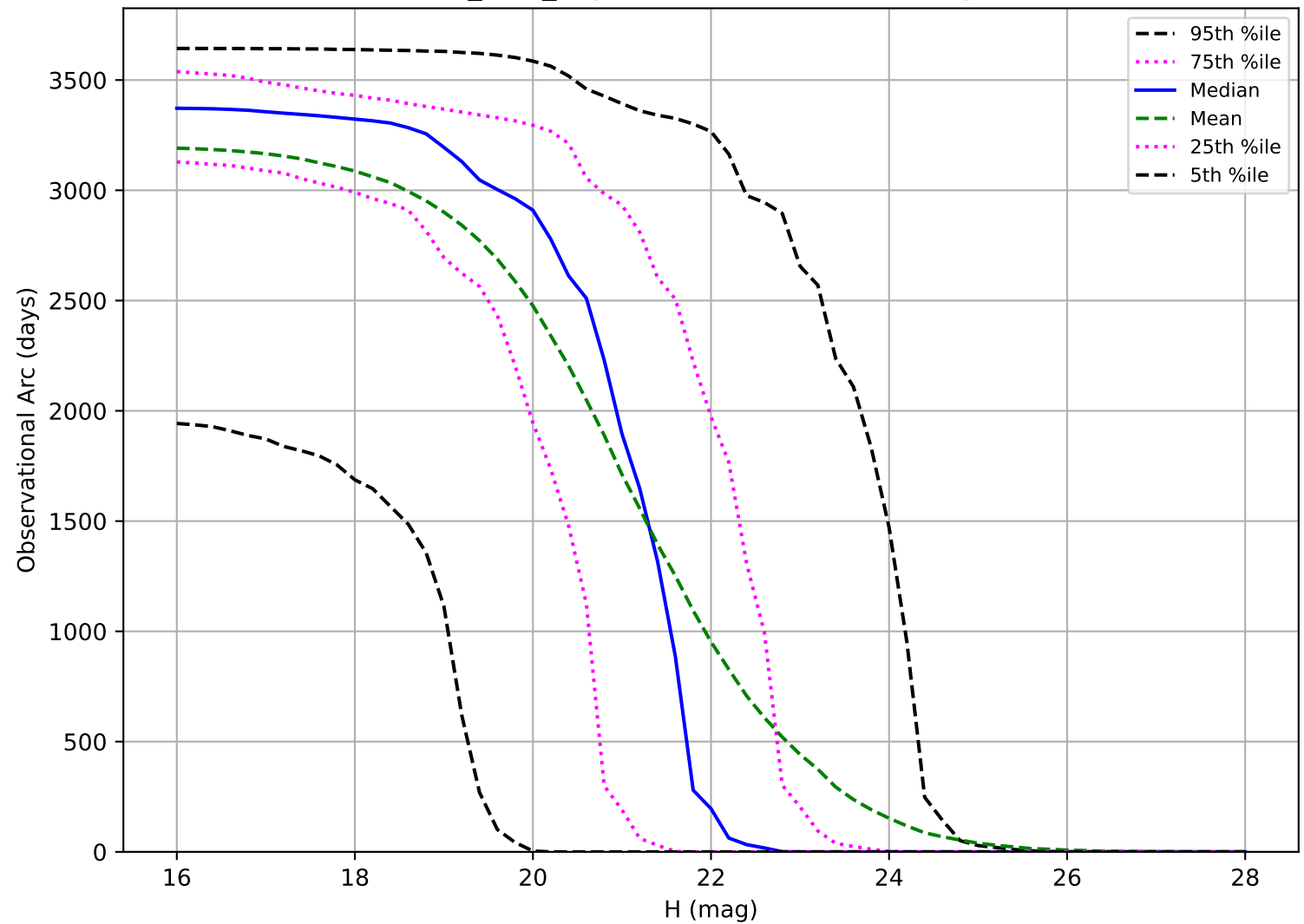
baseline_v3.6_10yrs: Observational Arc Length PHA
