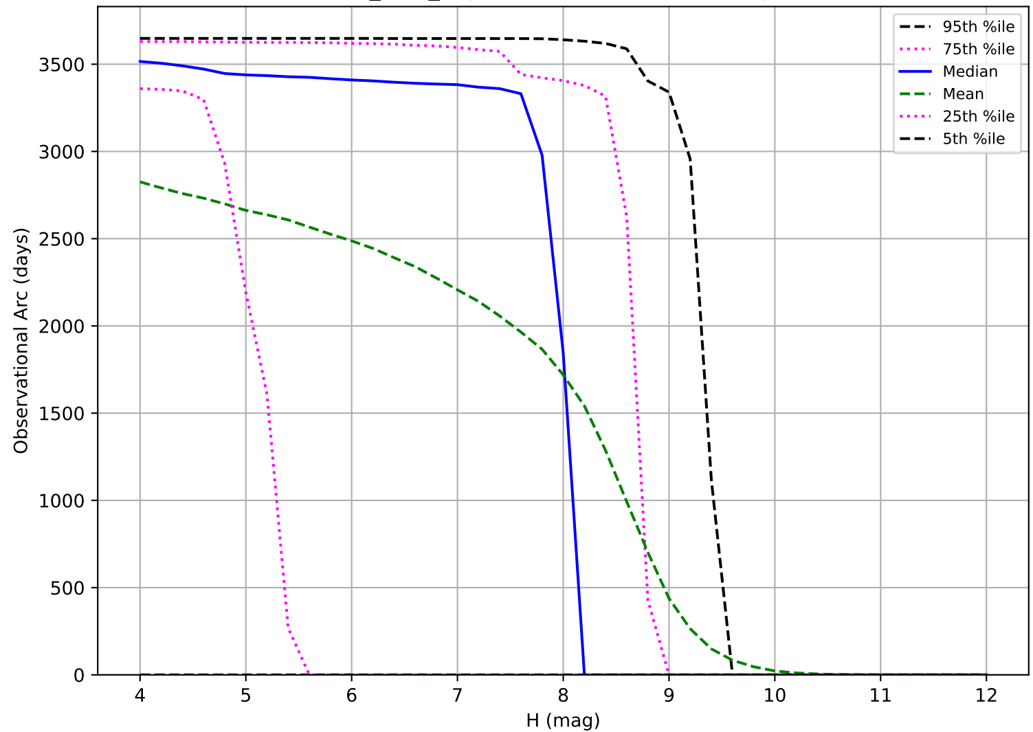
baseline_v3.6_10yrs: Observational Arc Length TNO
