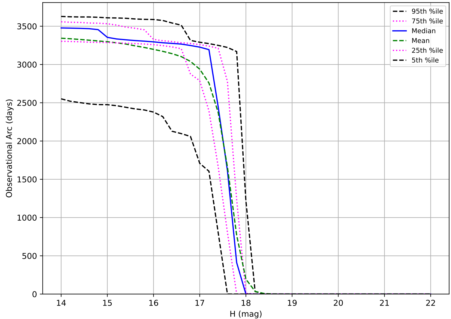
baseline_v3.6_10yrs: Observational Arc Length Trojan
