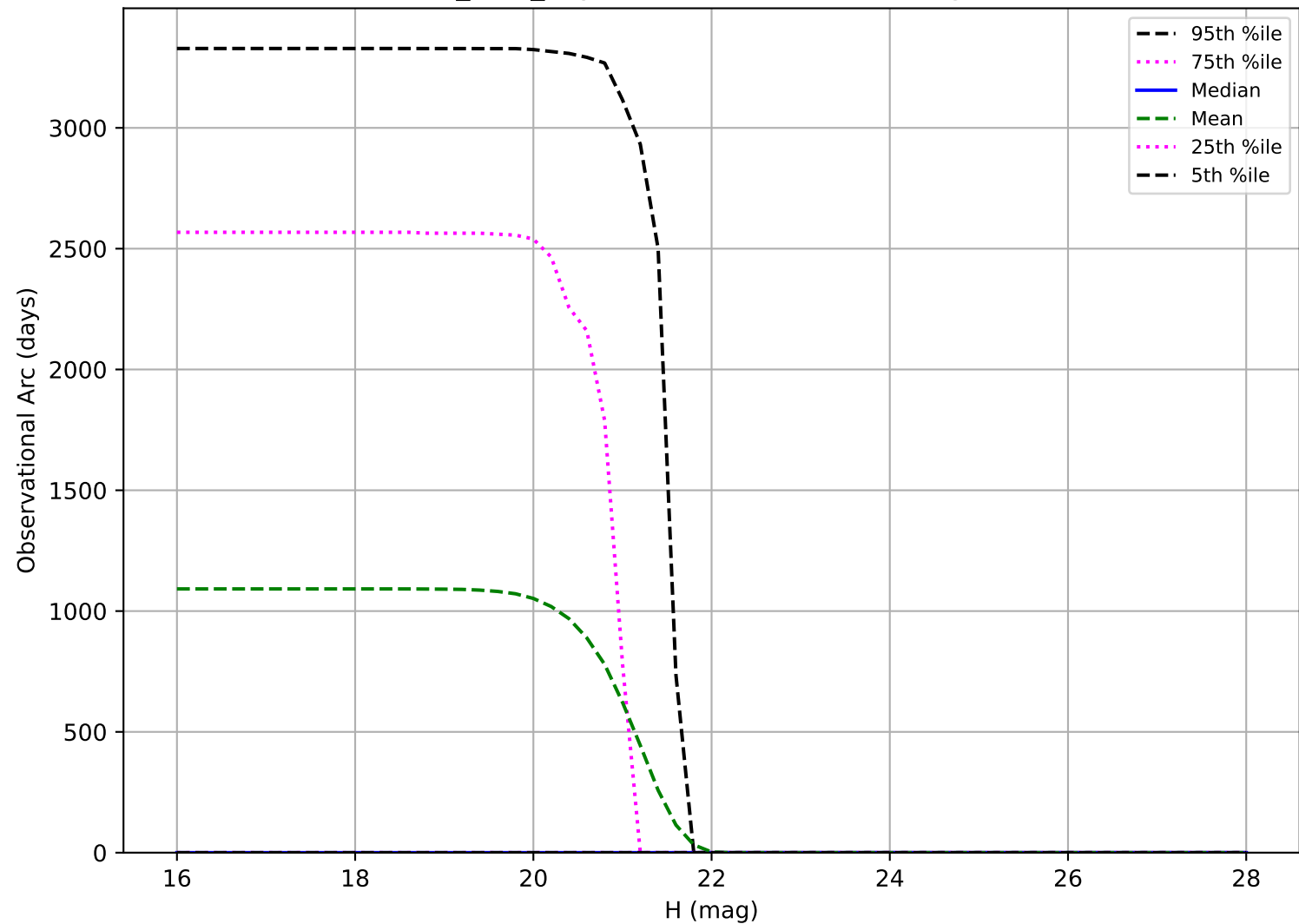
baseline_v3.6_10yrs: Observational Arc Length Vatira
