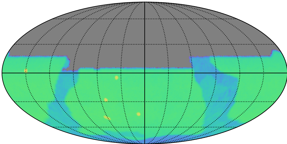
baseline_v4.0_10yrs y: CoaddM5
