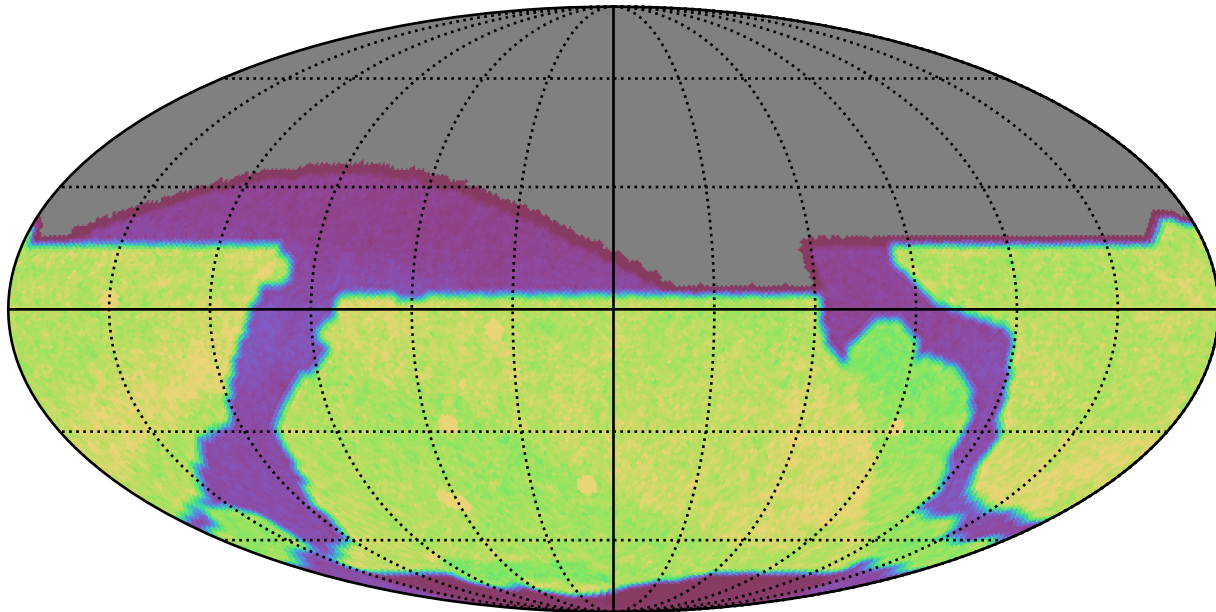
baseline_v4.0_10yrs : Count observationStartMJD
