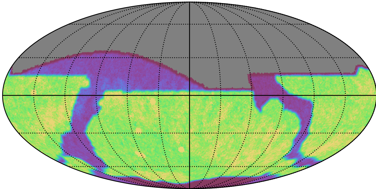
baseline_v4.0_10yrs r: Count observationStartMJD
