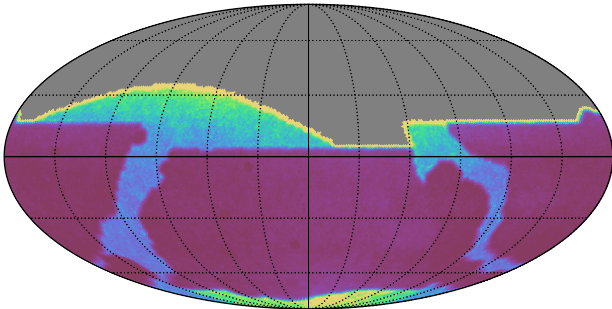
baseline_v4.0_10yrs : properMotion
