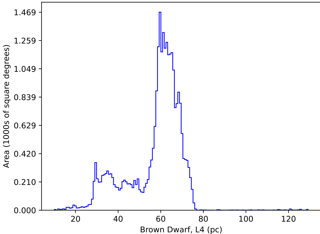
baseline_v4.0_10yrs : Brown Dwarf, L4
