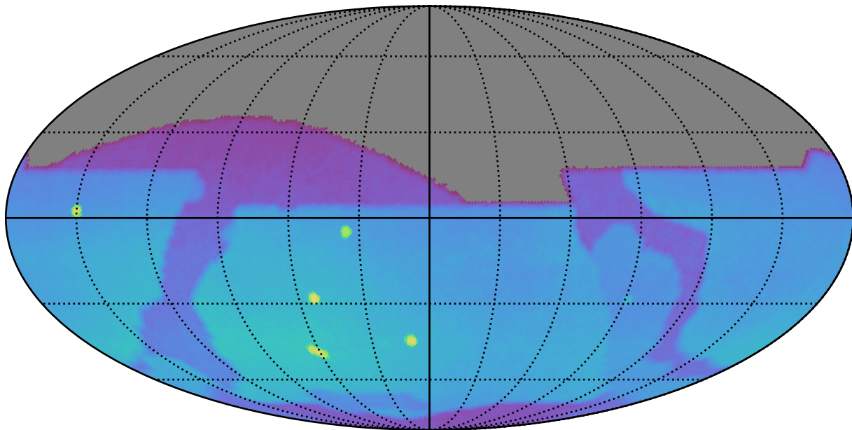
baseline_v4.0_10yrs : Brown Dwarf, L4
