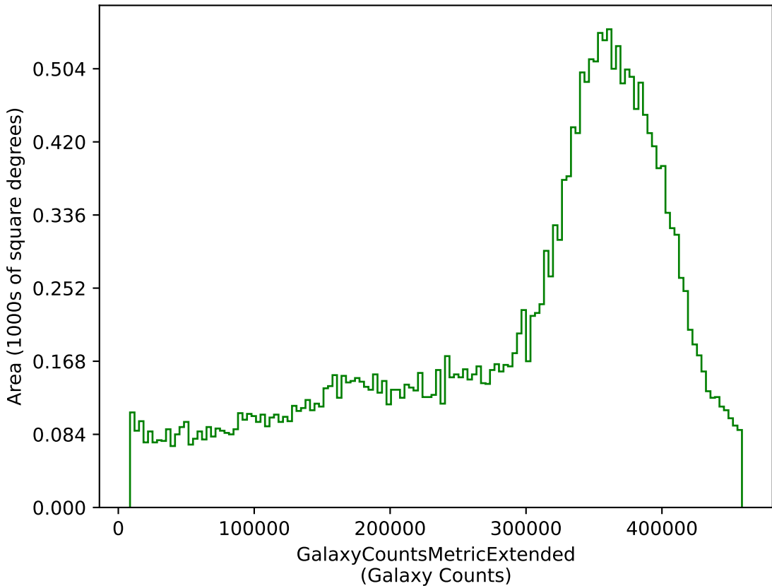
baseline_v4.0_10yrs g: GalaxyCountsMetricExtended
