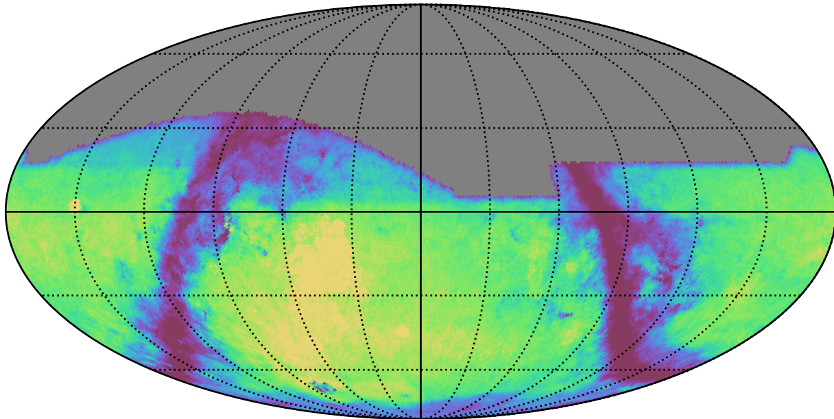
baseline_v4.0_10yrs g: GalaxyCountsMetricExtended
