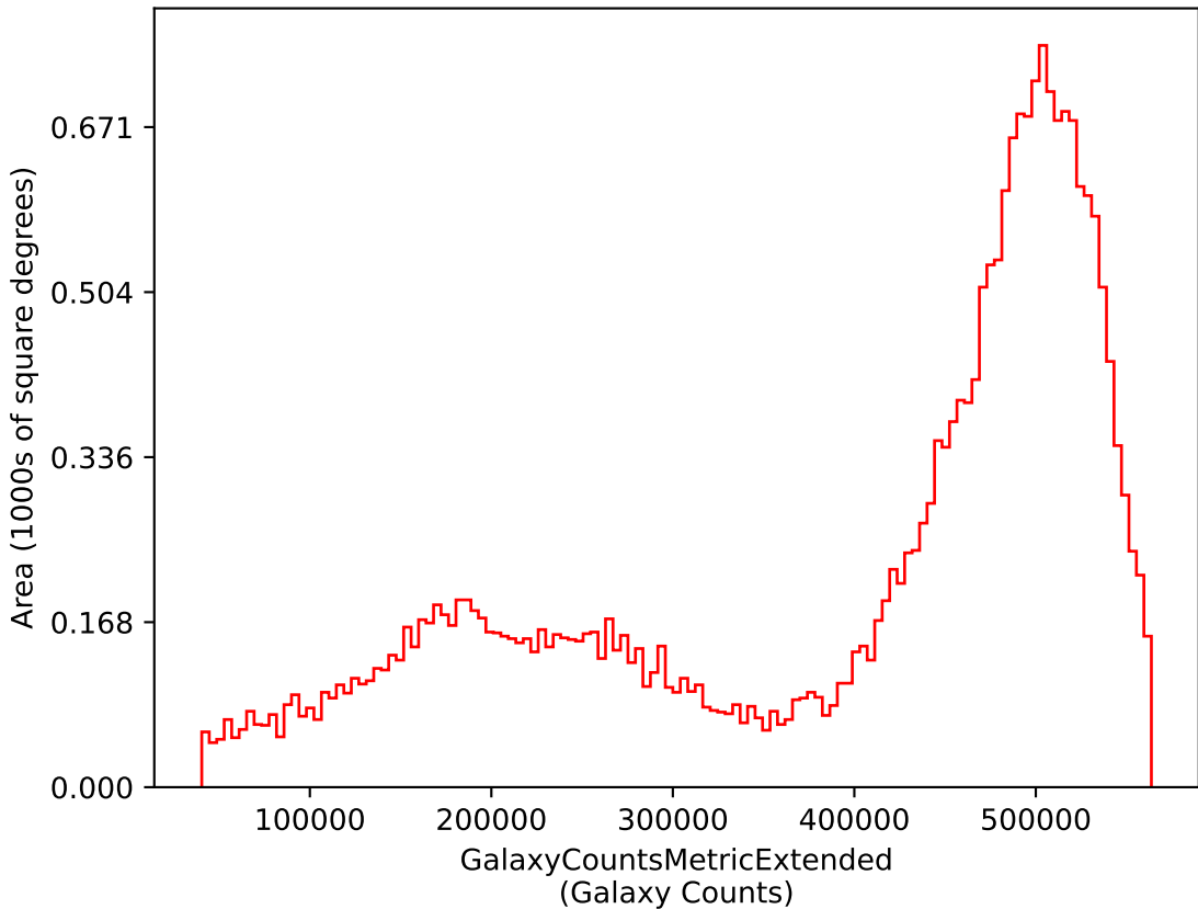
baseline_v4.0_10yrs i: GalaxyCountsMetricExtended
