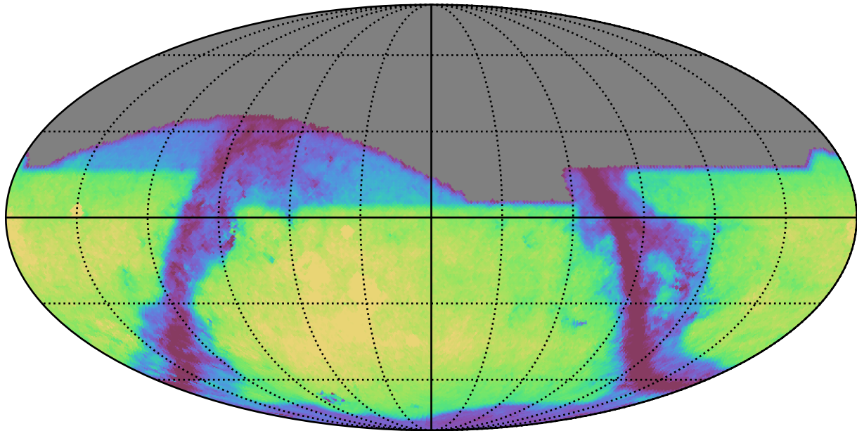
baseline_v4.0_10yrs i: GalaxyCountsMetricExtended
