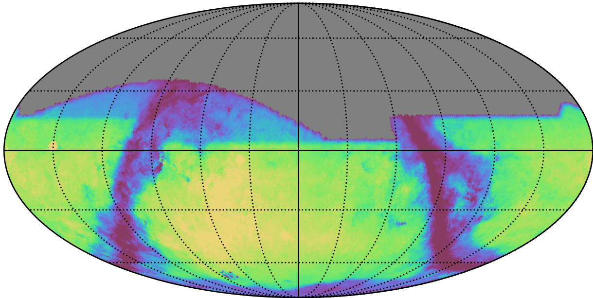
baseline_v4.0_10yrs r: GalaxyCountsMetricExtended
