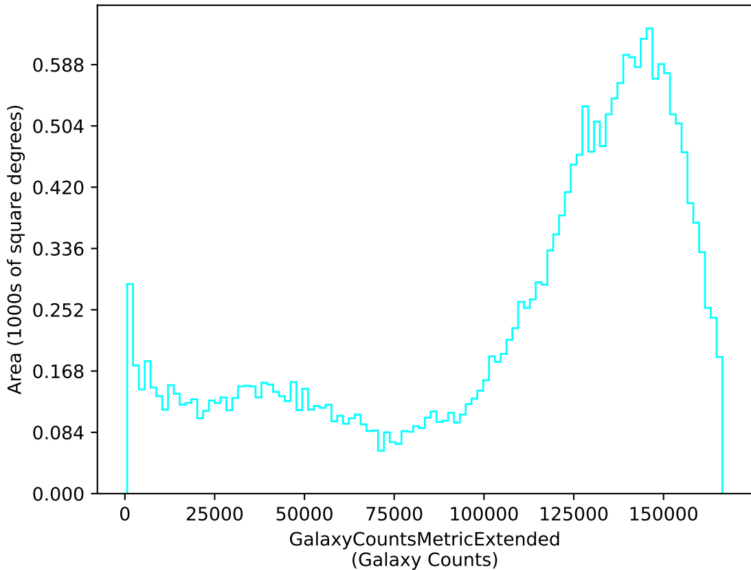
baseline_v4.0_10yrs u: GalaxyCountsMetricExtended
