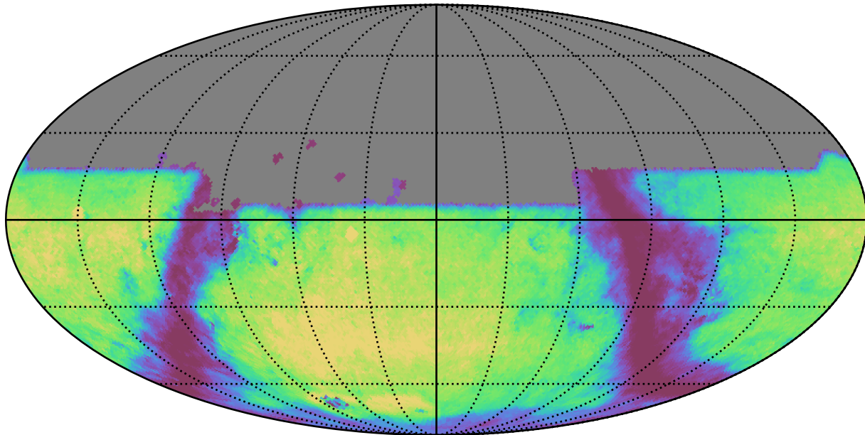
baseline_v4.0_10yrs u: GalaxyCountsMetricExtended
