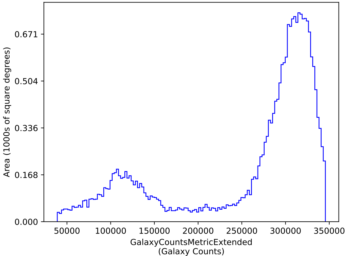
baseline_v4.0_10yrs y: GalaxyCountsMetricExtended
