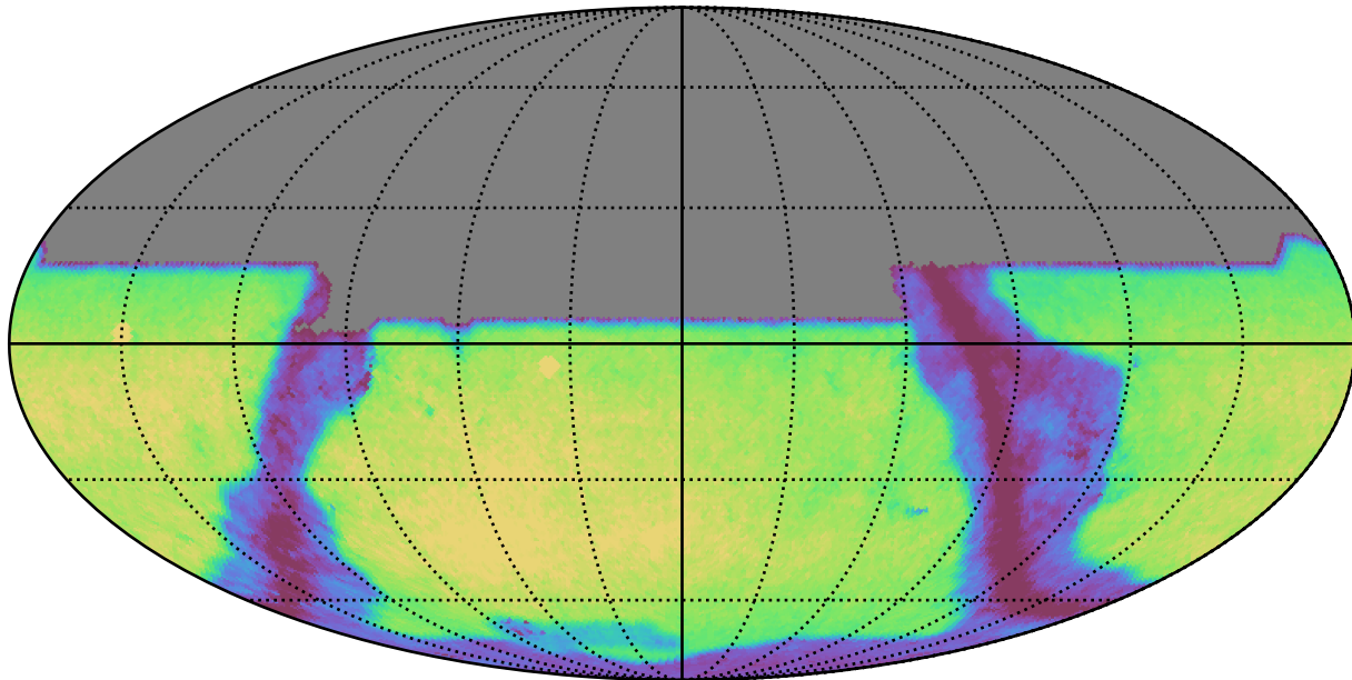
baseline_v4.0_10yrs y: GalaxyCountsMetricExtended
